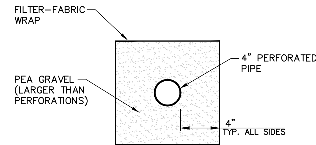
FOOTING DRAIN
