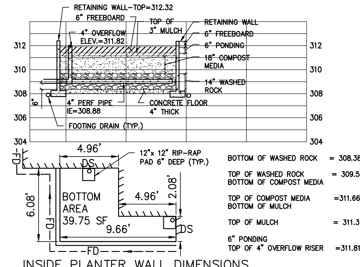
INSIDE PLANTER WALL DIMENSIONS
